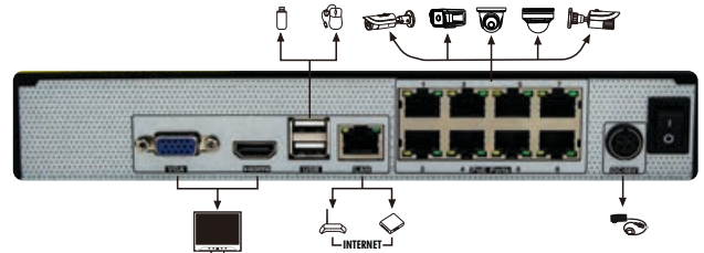
Rear Panel Interface for 8 Channel NVR
